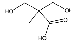
Bis-MPA
