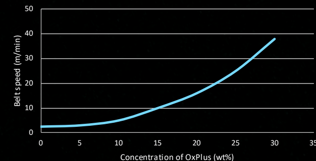
Surface cure (tack free)
