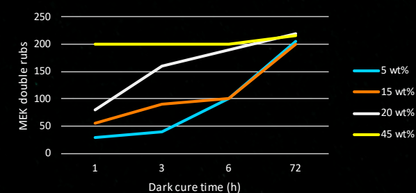
Through cure (chemical resistance)
